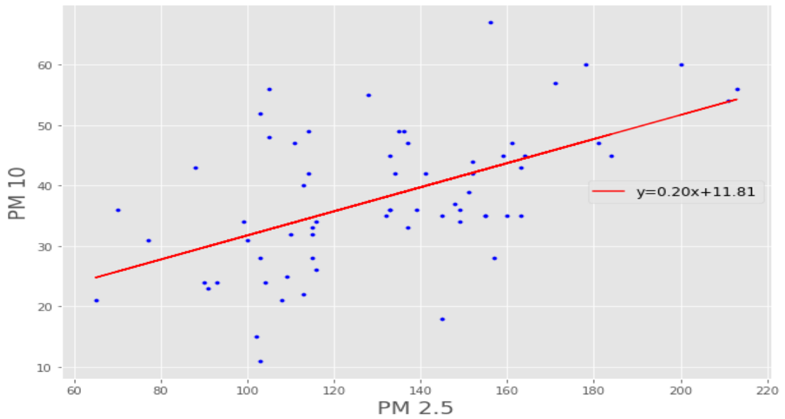
Fig 4.5. Regression of PM 2.5 and PM 10 before lockdown in US Embassy, Maharajgunj
