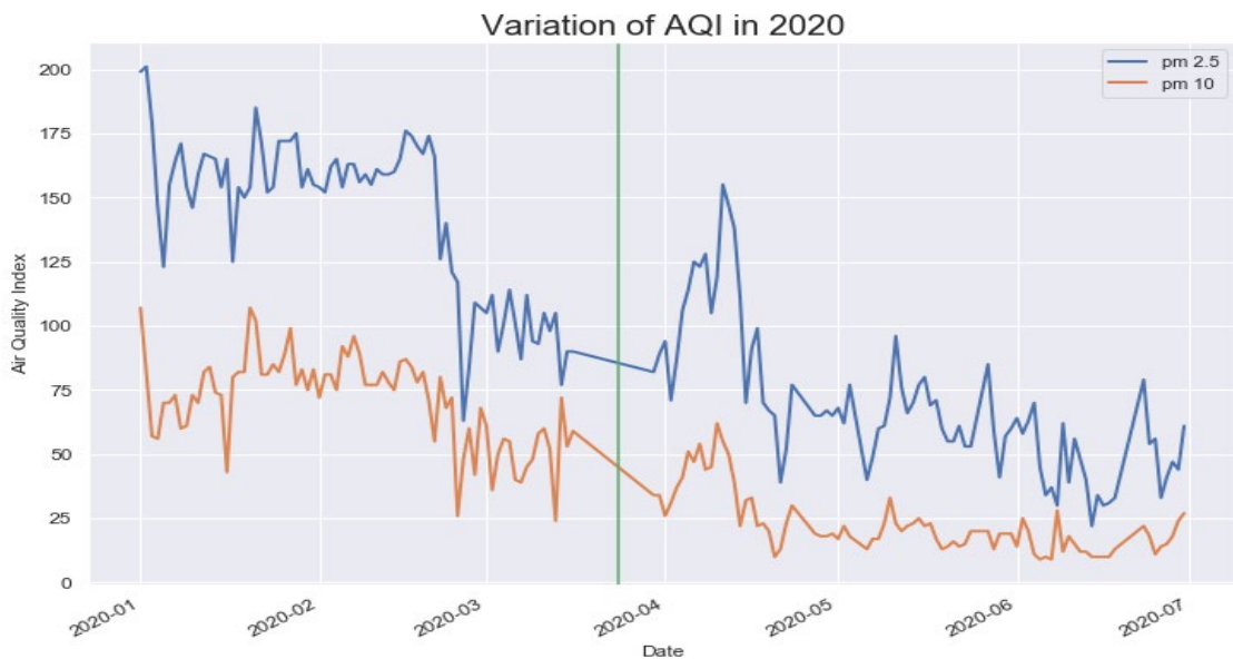
Fig (4.1) Air Quality Index variation in different date of 2020 on Ratnapark
