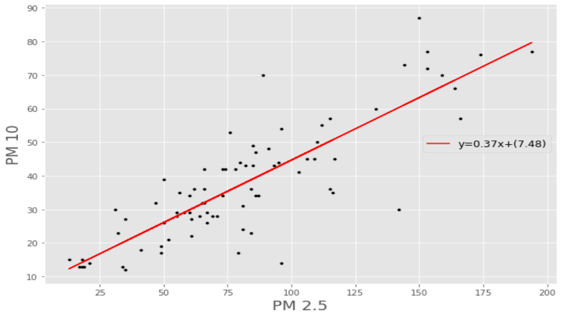
Fig 4.6. Regression of PM 2.5 and PM 10 during lockdown in US Embassy, Maharajgunj
