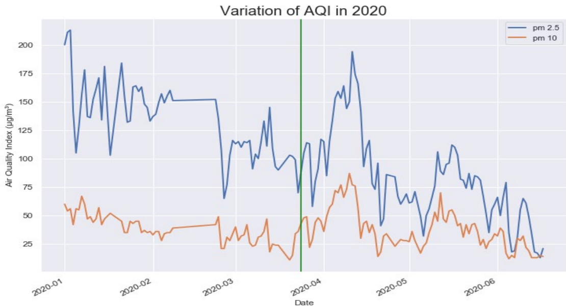
Fig (4.2) Air Quality Index variation in different date of 2020 on US Embassy, Maharajgunj
