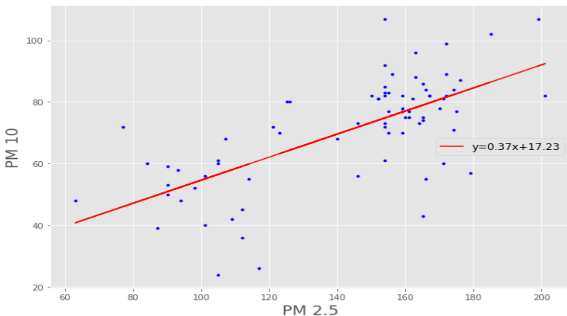
Fig 4.3. Regression of PM 2.5 and PM 10 before lockdown in Ratnapark
