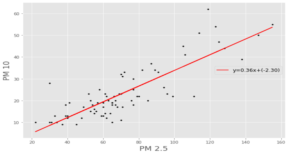
Fig 4.4. Regression of PM 2.5 and PM 10 during lockdown in Ratnapark
